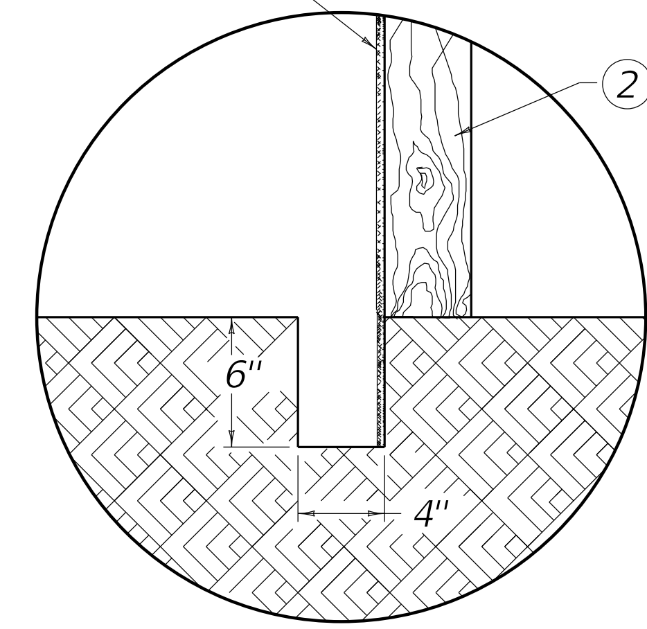
SECTIONAL DETAIL
